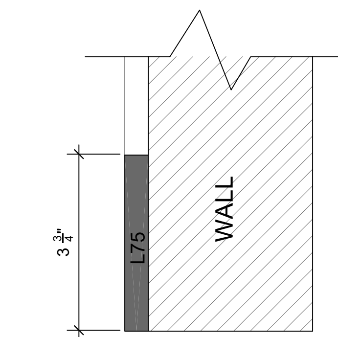
J-2 DETAIL, WALL J SCALE: HALF ACTUAL SIZE
