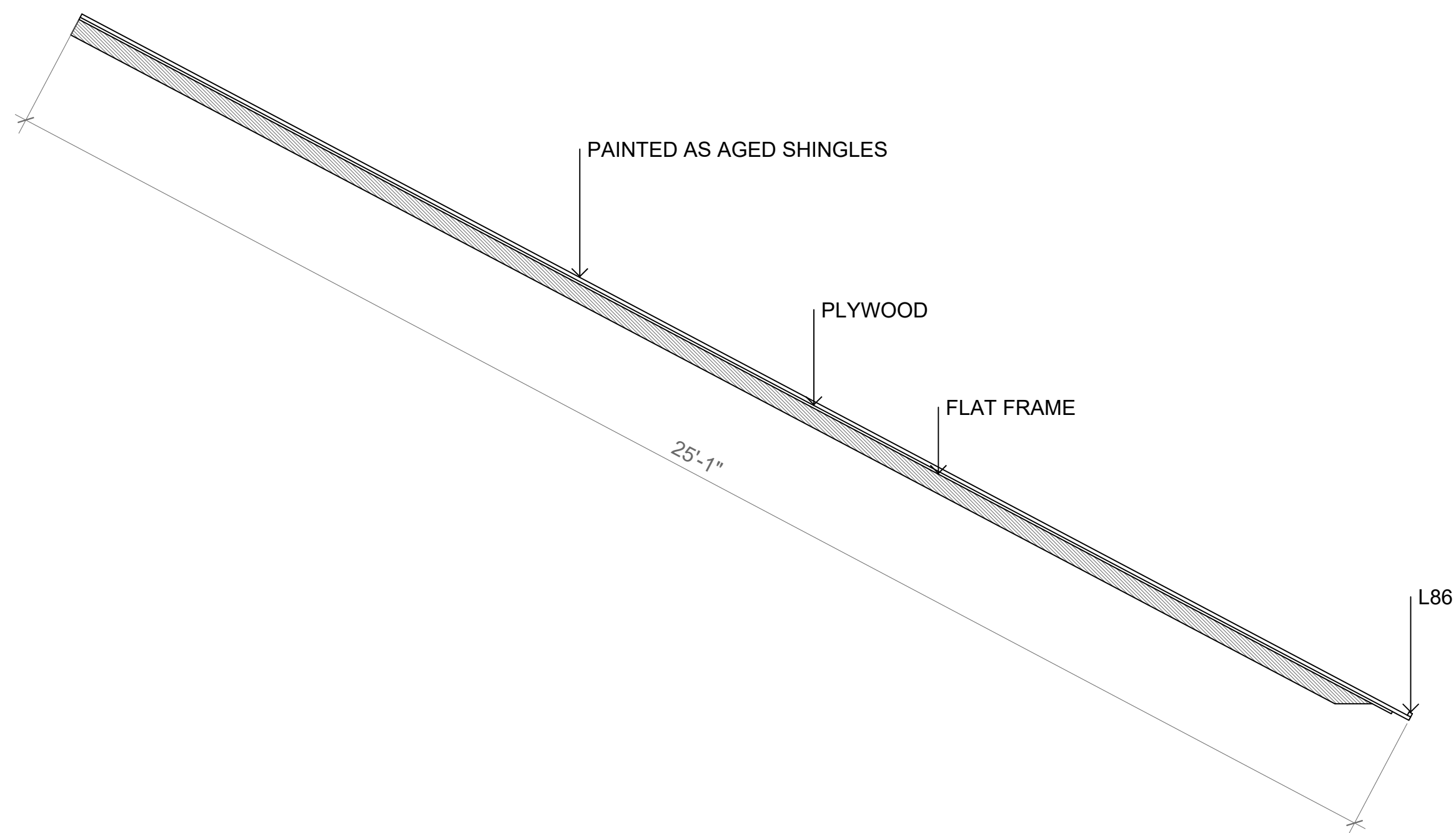
H-3 SECTION THROUGH SLOPED ROOF SCALE: 1/2" = 1'-0"
