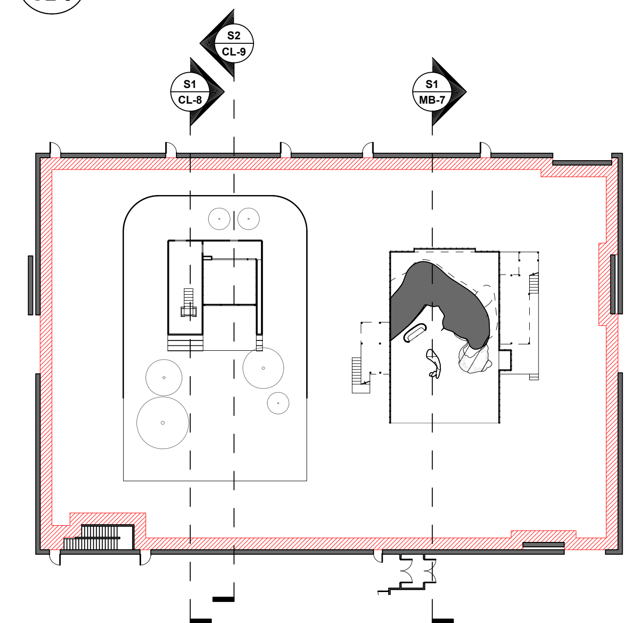
RP REFERENCE PLAN CL-9 SCALE: 1/32" = 1'-0"
