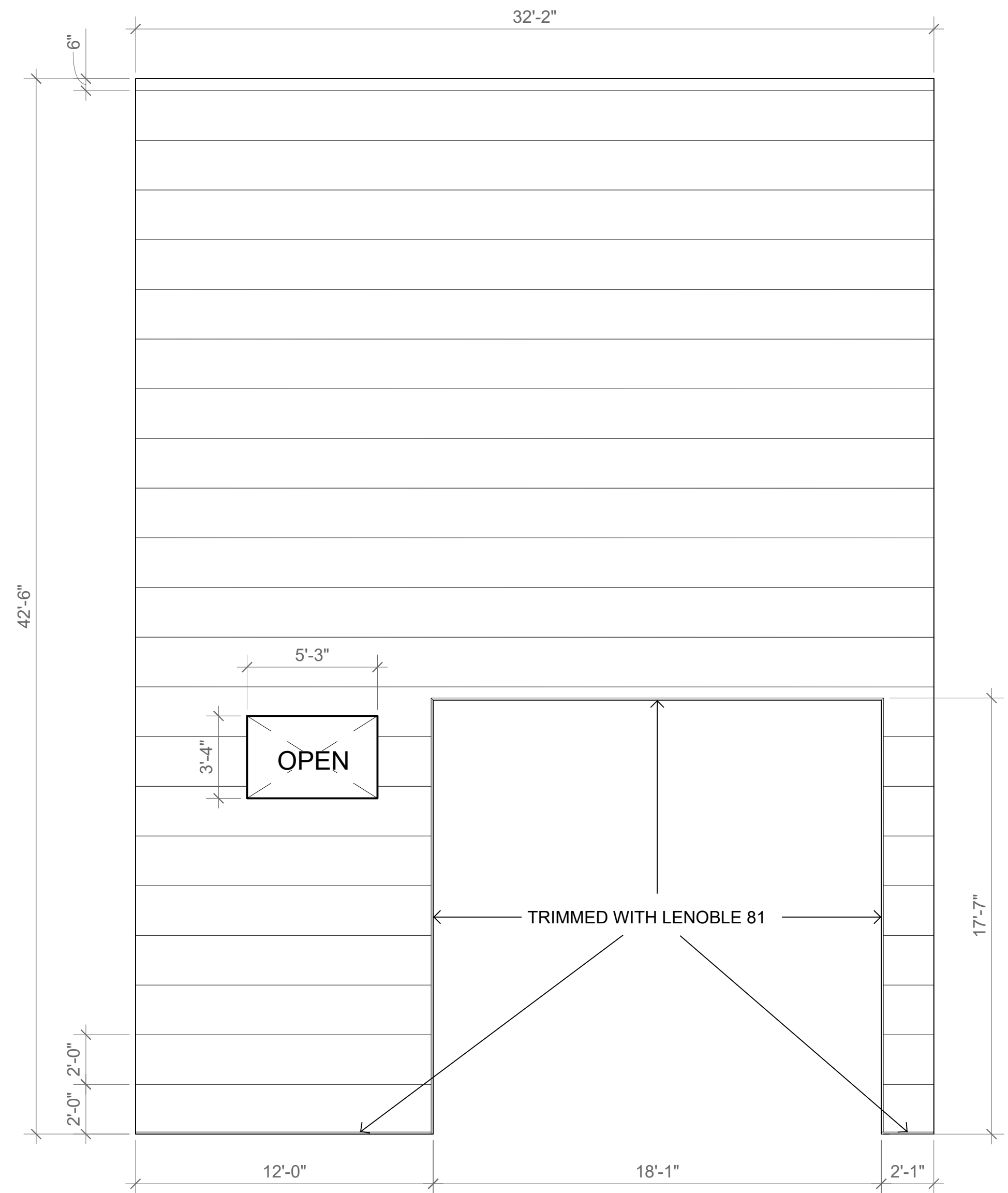
H-1 ELEVATION PARALLEL TO SLOPE ANGLE SCALE: 1/4" = 1'-0"
