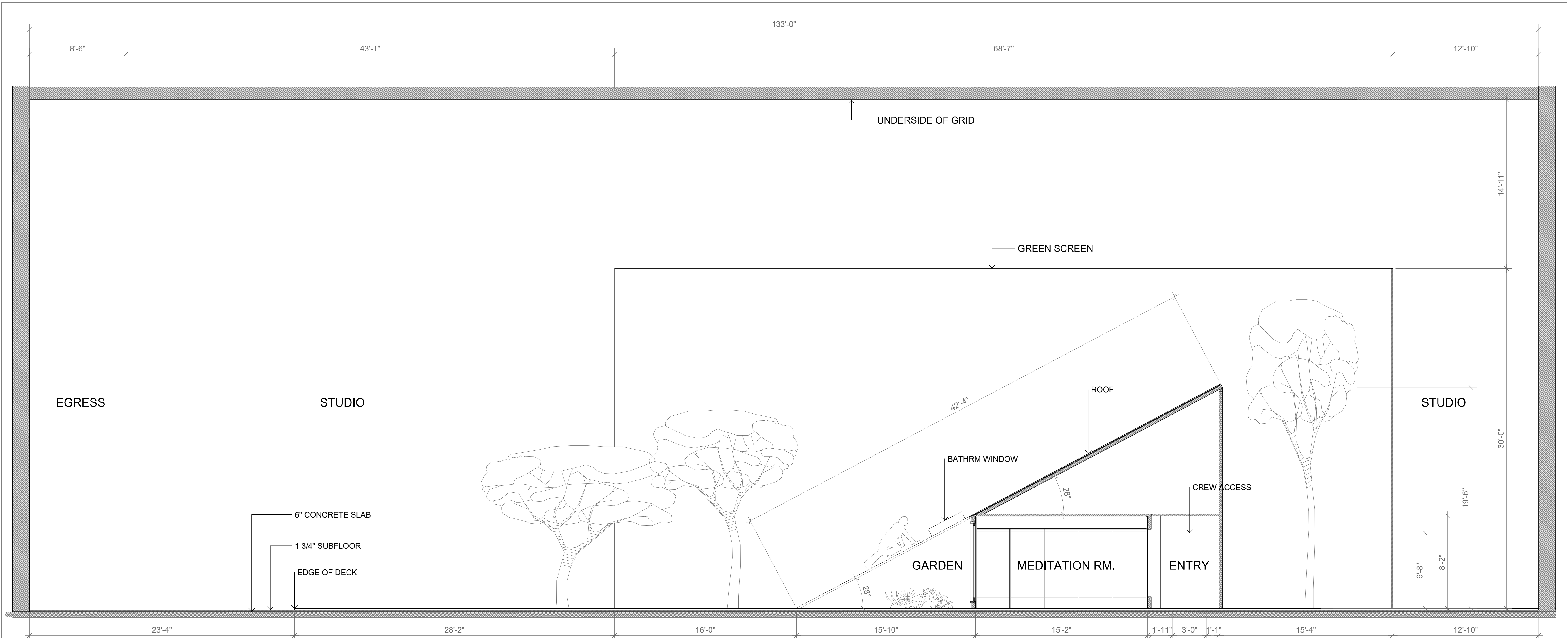
S2 SECTION THROUGH CATLADY SET CL-9 SCALE: 1/4" = 1'-0"
