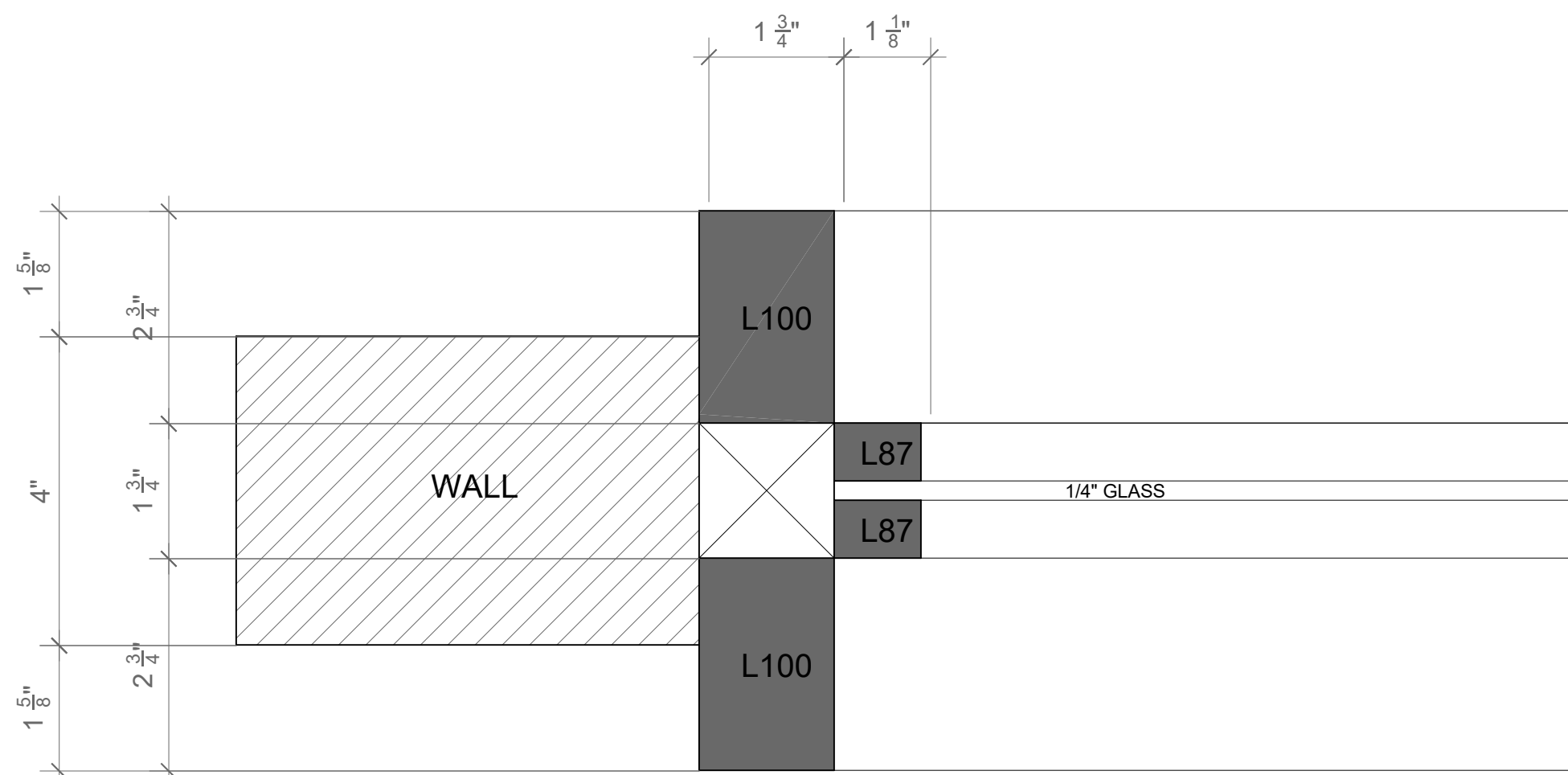
DT-3 WINDOW DETAIL, PLAN CL-16 SCALE: HALF ACTUAL SIZE
