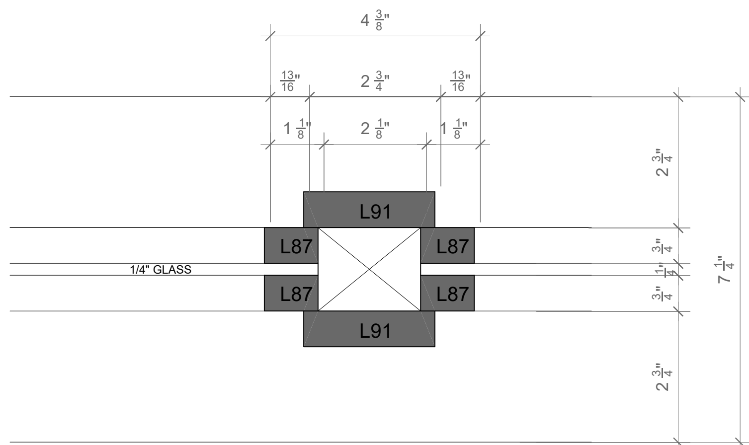
DT-4 WINDOW DETAIL, PLAN CL-16 SCALE: HALF ACTUAL SIZE
