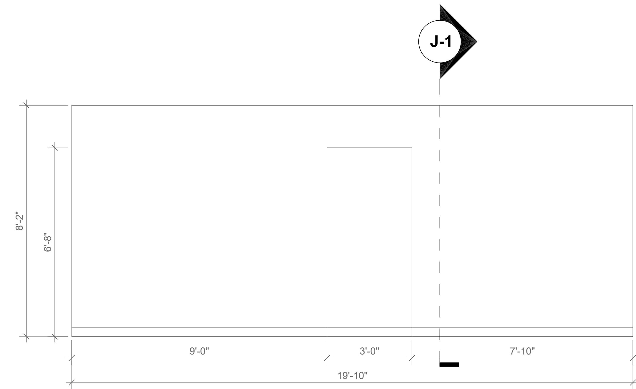
J ELEVATION, ENTRY WALL J SCALE: 1/2" = 1'-0"
