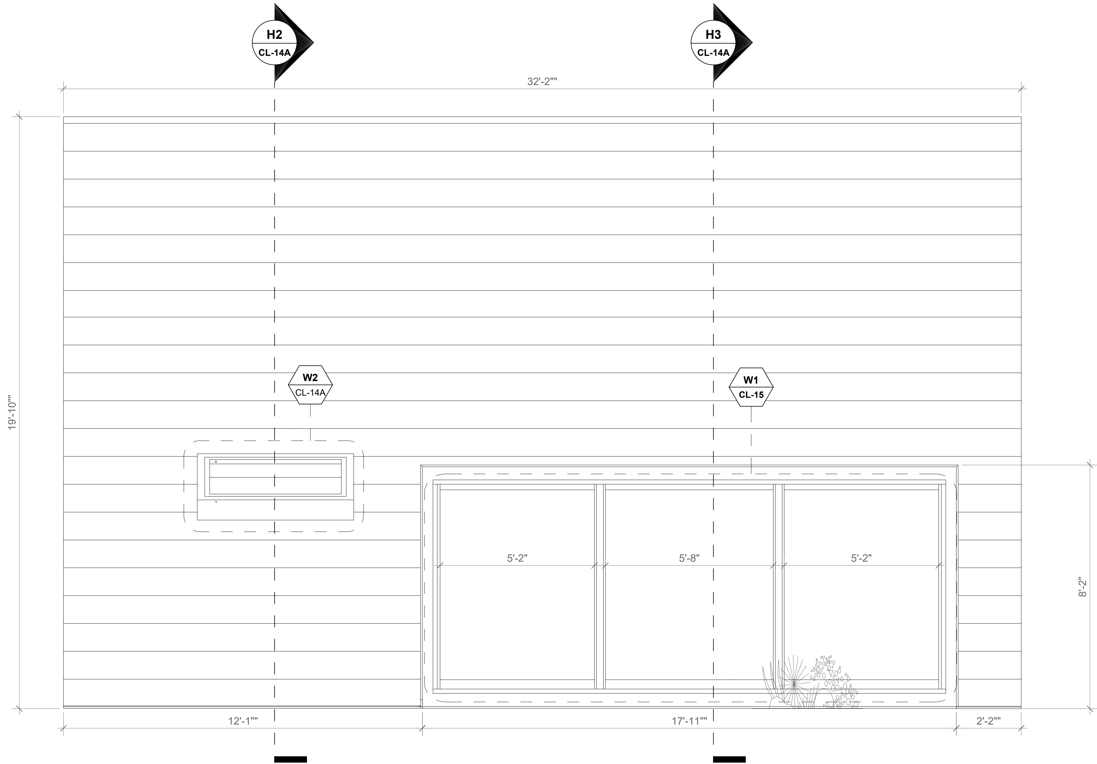
H ELEVATION, SLOPED ROOF SCALE: 1/2" = 1'-0"
