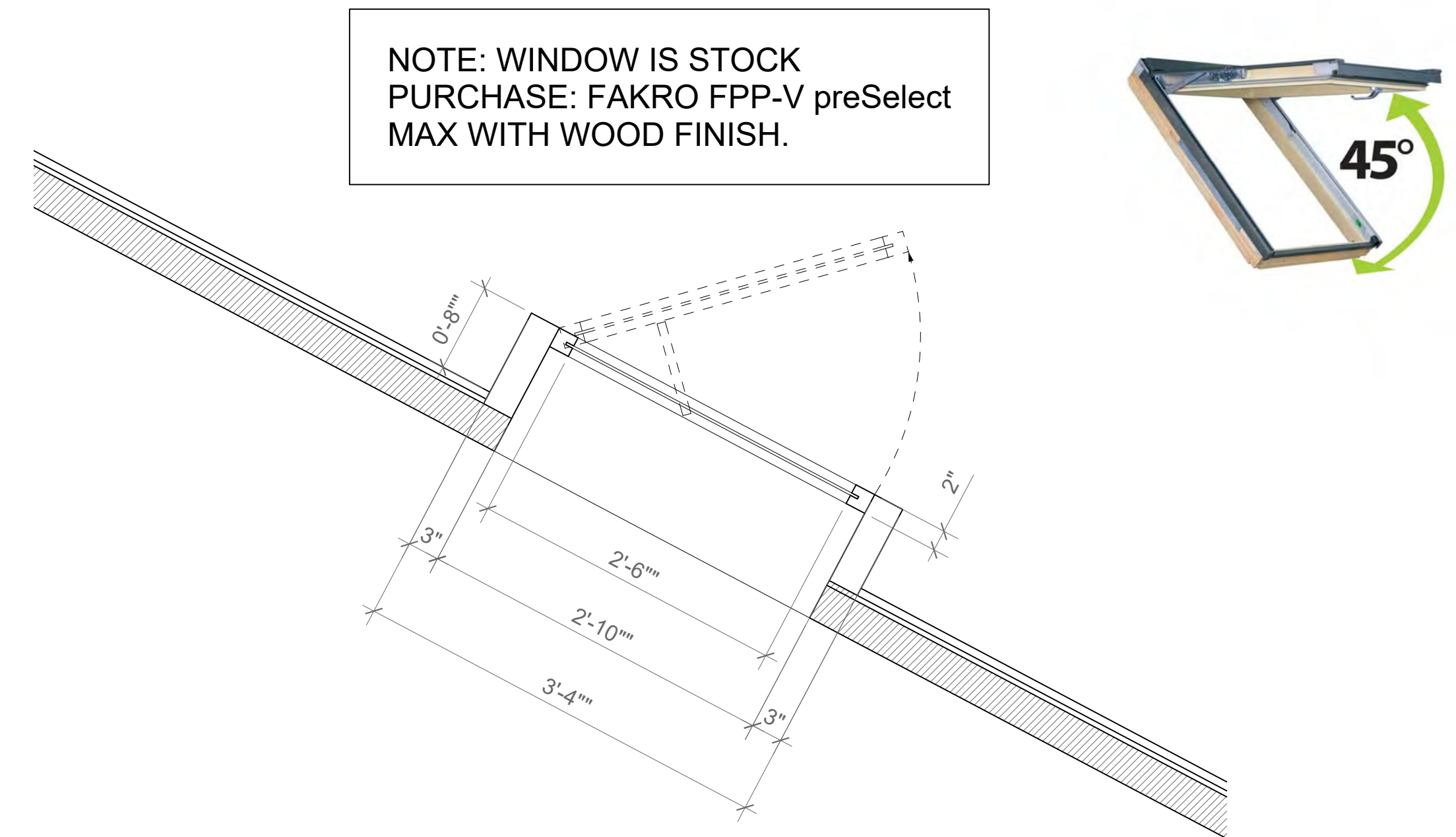
W2 WINDOW DETAIL CL-14A SCALE: 1" = 1'-0"
